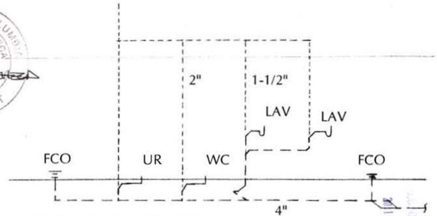
Men's Room Sanitary Riser Diagram
