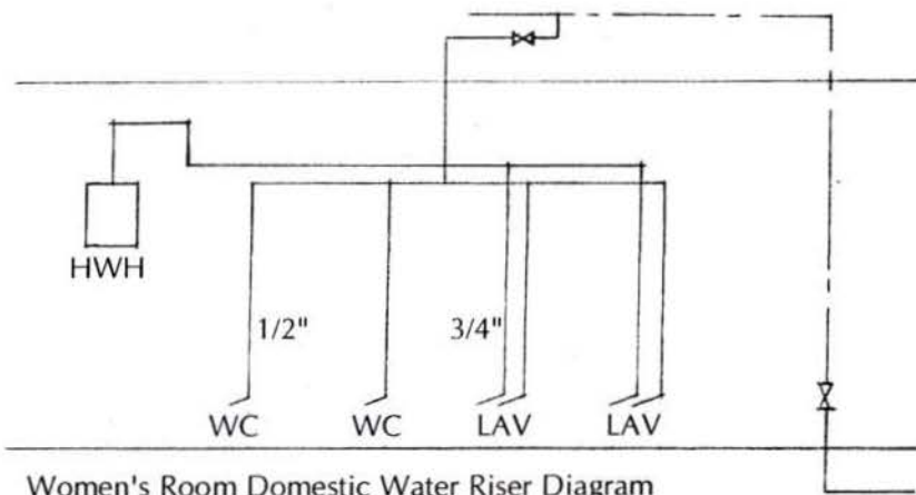
Women's Room Domestic Water Riser Diagram
