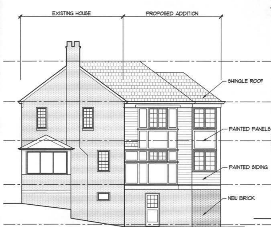
PROPOSED SOUTH-WEST ELEVATION
