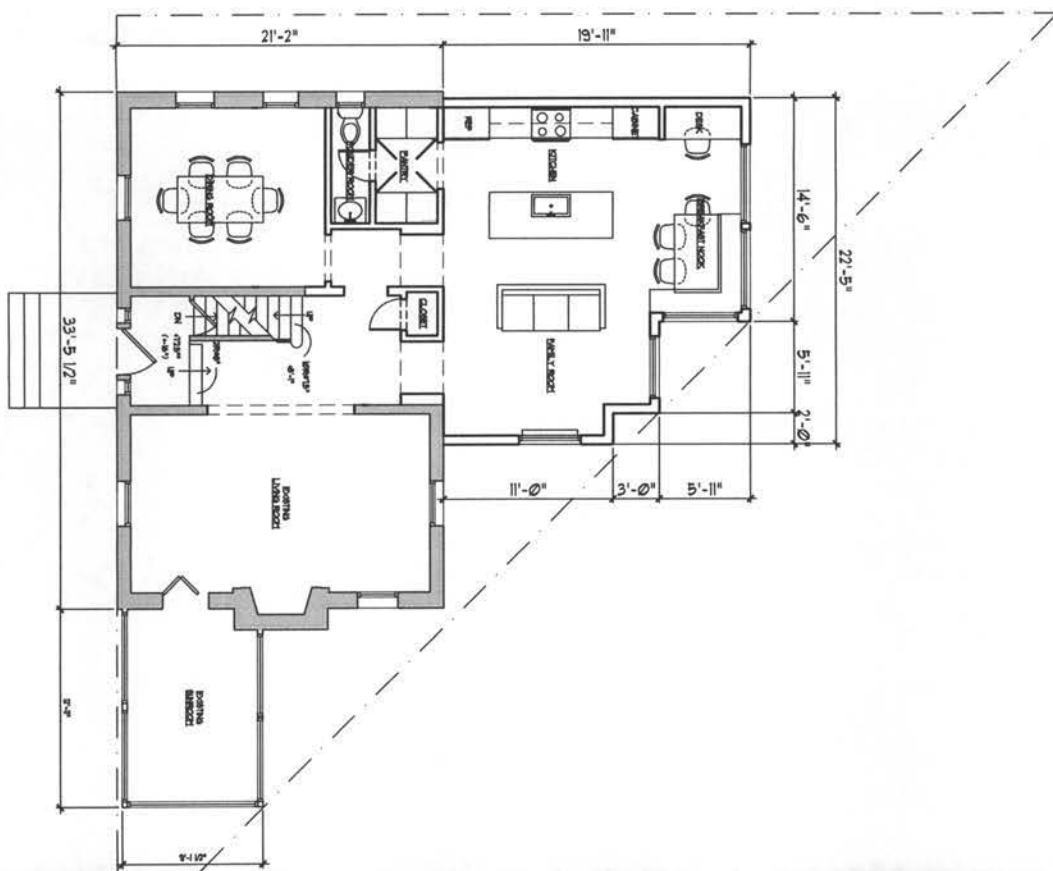
FIRST FLOOR PLAN 1/8" = 1'-0"
