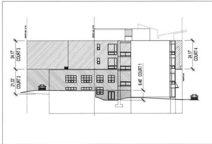
NORTH ELEVATION
