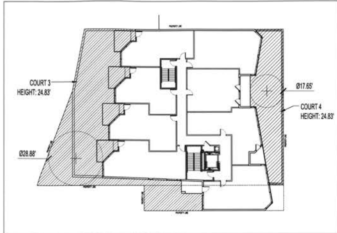
THIRD/FOURTH FLOOR PLAN
