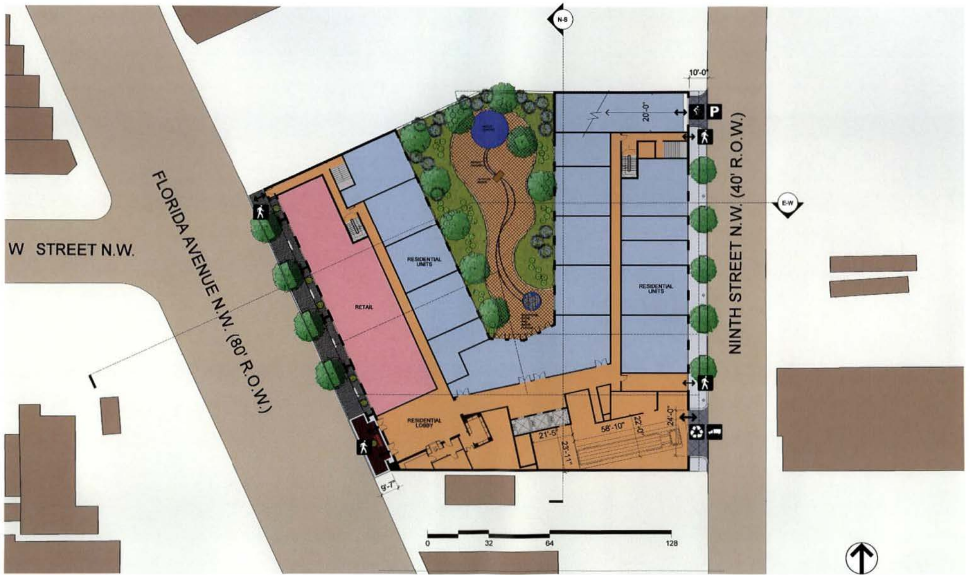
Ground Floor Plan Approved 3/2/06
